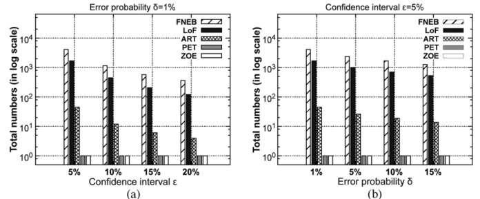
Fig. 14. Memory overhead in storing the random numbers: (a) with different confidence interval \epsilon , and the same error probability \delta = 1\% ; (b) with different error probability \delta , and the same confidence interval \epsilon = 5\% .
