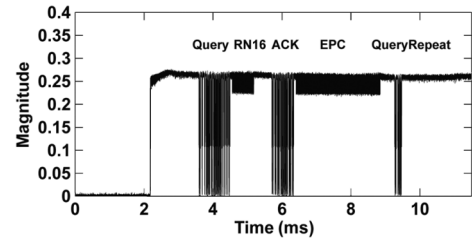
Fig. 6. Communication between reader and tag in the inventory communication. The Query command is sent by the reader at around 4 ms followed by the reply of RN16 from a tag. The ACK is sent at around 6 ms followed by the EPC code from the tag. The QueryRepeat is sent to query other tags.
