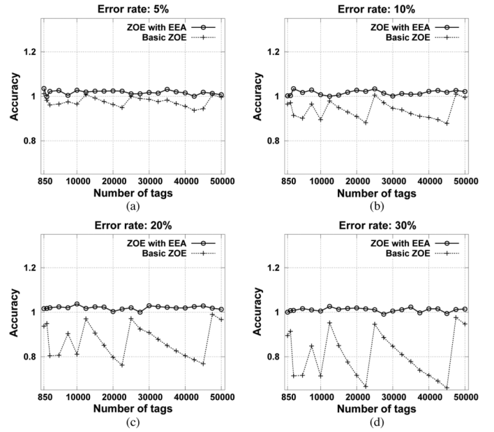
Fig. 10. Evaluation of estimation accuracy under different error rates: (a) error rate = 5%; (b) error rate = 10%; (c) error rate = 20%; (d) error rate = 30%.
