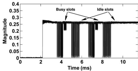
Fig. 7. Communication between reader and tag in the ZOE protocol. The first Count command is sent at around 4 ms followed by a busy slot. The second Count command is followed by an empty slot.
