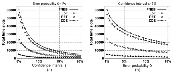
Fig. 12. Performance comparison: (a) protocol performance with different confidence interval \epsilon , and the same error probability \delta = 1\% ; (b) protocol performance with different error probability \delta and the same confidence interval \epsilon = 5\% .
