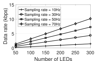
Fig. 19: The data rate without LED failures
