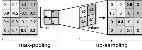
Figure 7: Up-pooling diagram.
