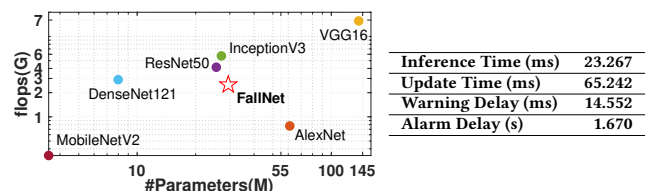
(a) FallNet model complexity compared with (b) Latency of SiFall components.
