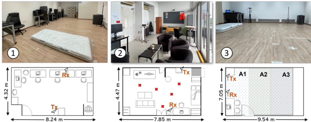
Figure 8: The environment of the three testbeds and their floor plans.
