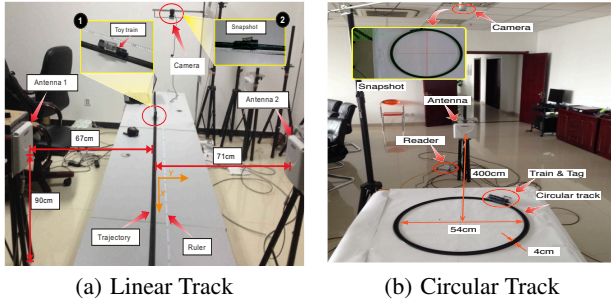
Figure 7: Experiment setups
