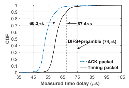
Figure 7: CDF of measured delay of the SWAN ACK and timing packet.
